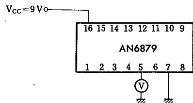
Test Circuit 3 ( V_{REF} )
