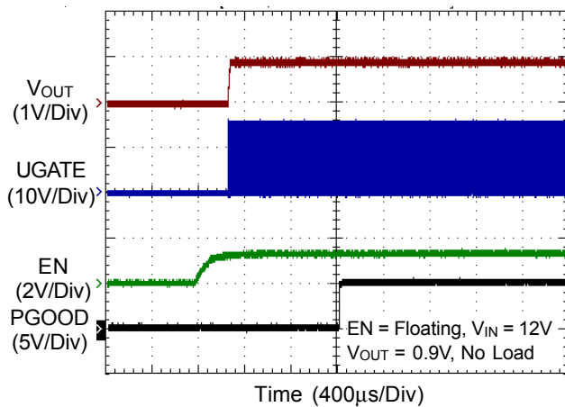
Power On From EN (CCM)
