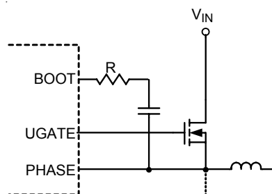
Figure 8. Reducing the UGATE Rise Time
