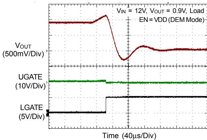
OVP Waveforms
