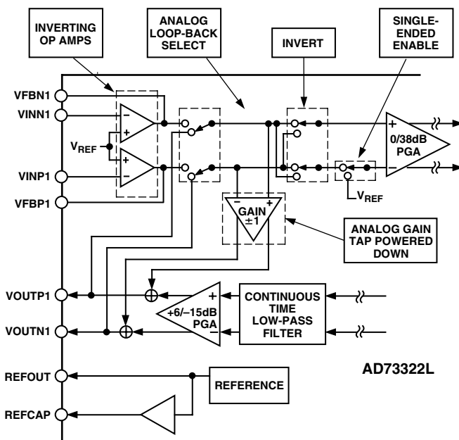
Figure 13. Analog Loop-Back Connectivity
