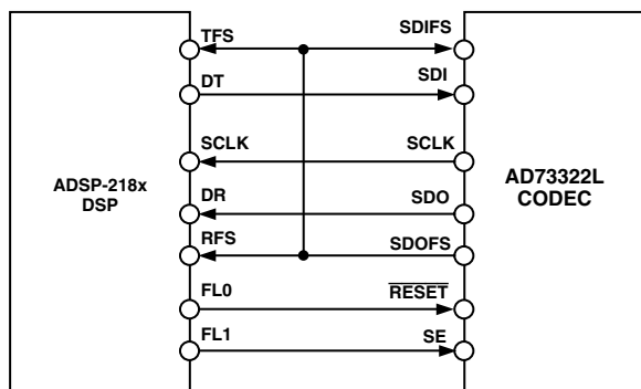
Figure 34. AD73322L Connected to ADSP-218x
