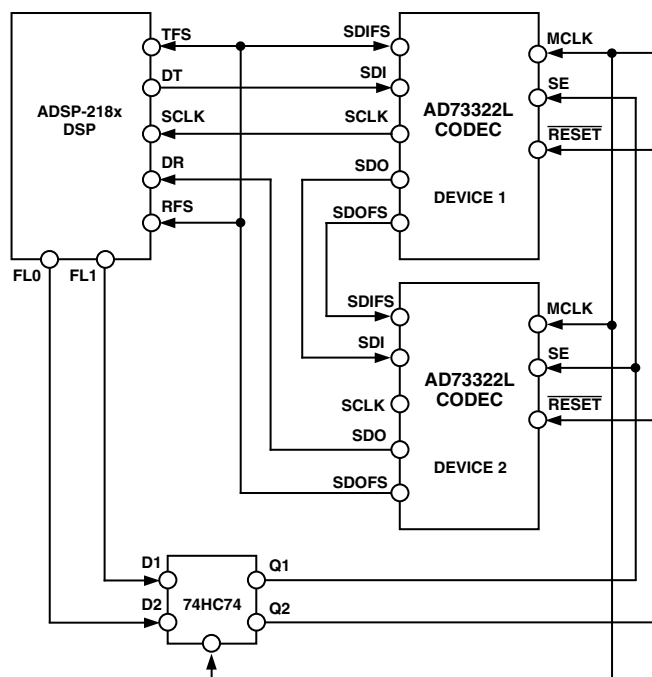
Figure 37. Connection of Two AD73322Ls Cascaded to ADSP-218x
