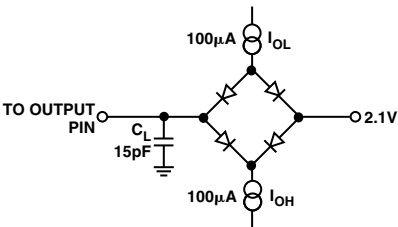
Figure 2. Load Circuit for Timing Specifications
