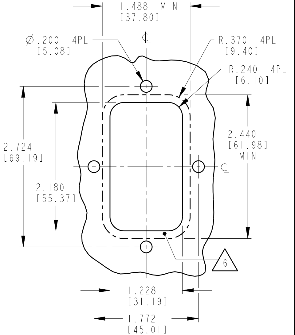
RECOMMENDED CUTOUT
