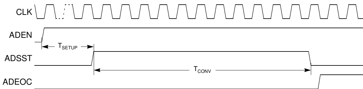
Figure 39. Timing Diagram
