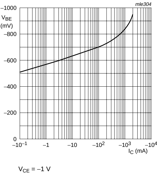
Fig 9. BCP69-25: Base-emitter voltage as a function of collector current; typical values
