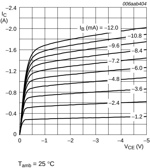
Fig 8. BCP69-25: Collector current as a function of collector-emitter voltage; typical values
