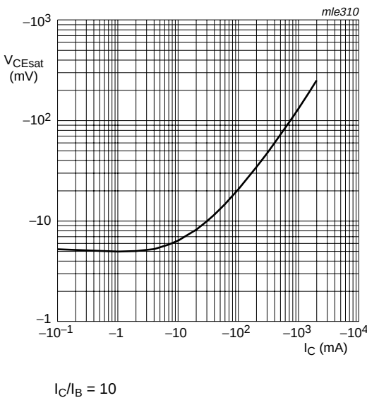
Fig 10. BCP69-25: Collector-emitter saturation voltage as a function of collector current; typical values
