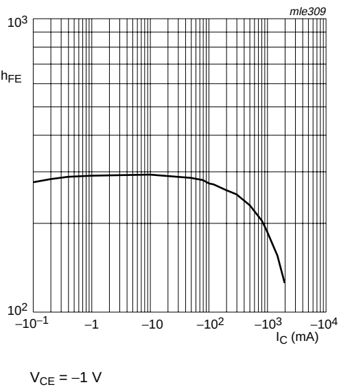
Fig 7. BCP69-25: DC current gain as a function of collector current; typical values
