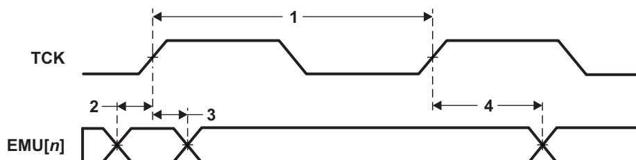
Figure 8-47. HS-RTDX Timing
