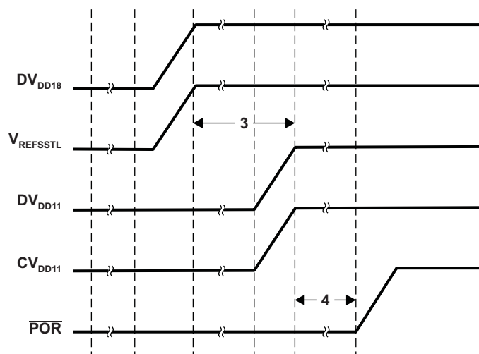
Figure 8-4. Power-Supply Timing
