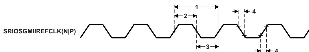
Figure 8-43. SRIOSGMIIREFCLK(N|P) Timing
