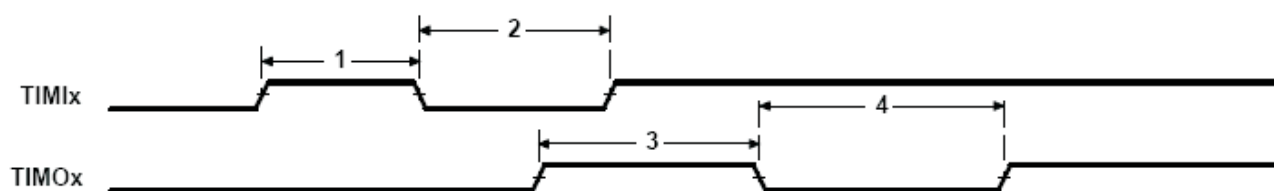
Figure 8-42. Timer Timing
