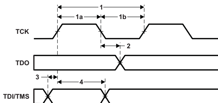
Figure 8-46. JTAG Timing
