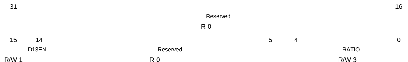
Figure 8-14. PLL Controller Divider 13 Register (PLLDIV13) [Hex Address: 029A 0184]
