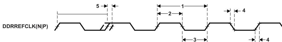
Figure 8-22. DDRREFCLK(N|P) Timing
