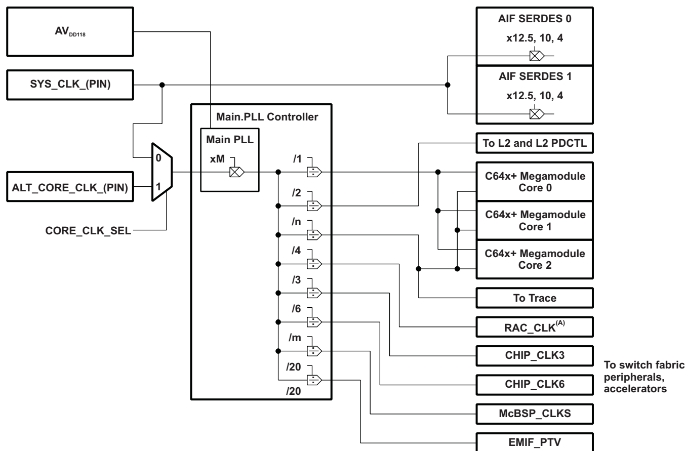
Figure 8-10. PLL Controller Diagram
