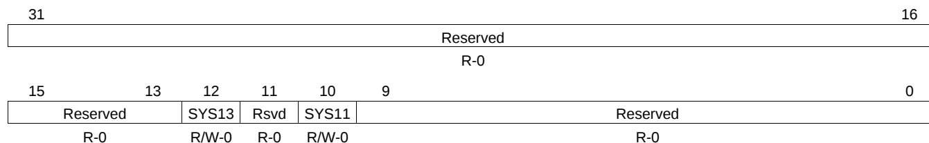
Figure 8-18. PLLDIV Divider Ratio Change Status Register (DCHANGE) [Hex Address: 029A 0144]
