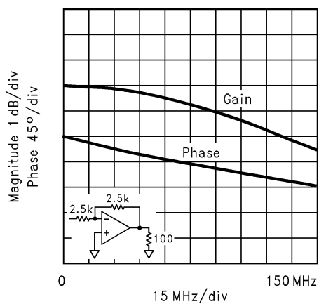
Frequency Response, A_V = -1 , R_f = 2.25k\Omega
