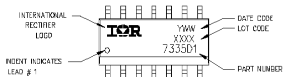
TOP MARKING
