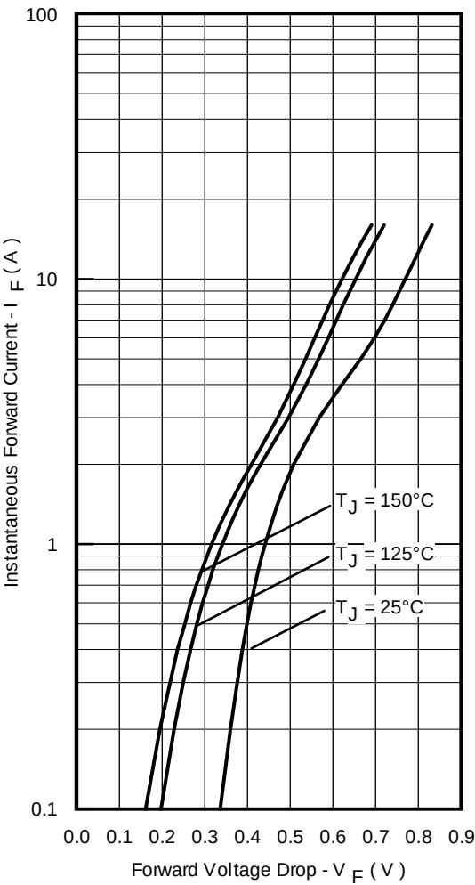
Fig. 29 - Maximum Forward Voltage Drop Characteristics
