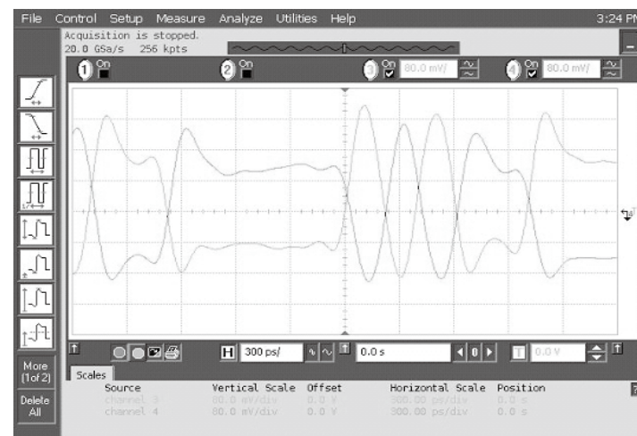
Data Waveforms, 3.0Gbps (left) & 6.0Gbps (right)
