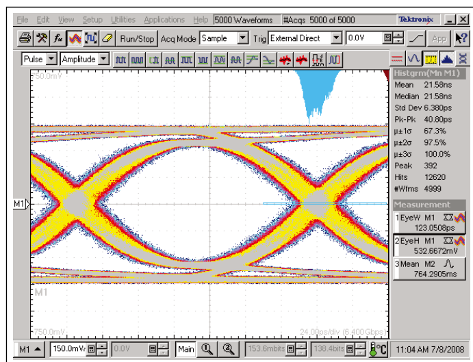
Output Eye
