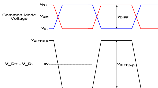
Definition of Differential Voltage and Differential Voltage Peak-to-Peak
