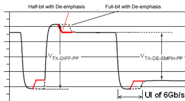
Definition of Pre-de-emphasis
