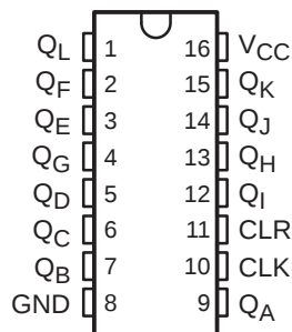
SN54LV4040A . . . J OR W PACKAGE SN74LV4040A . . . D, DB, DGV, NS, OR PW PACKAGE (TOP VIEW)
