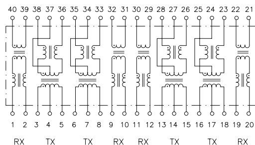
Circuit D
