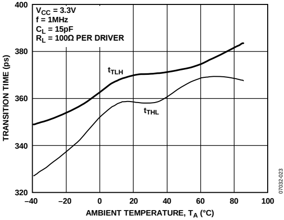
Figure 23. Transition Time vs. Ambient Temperature
