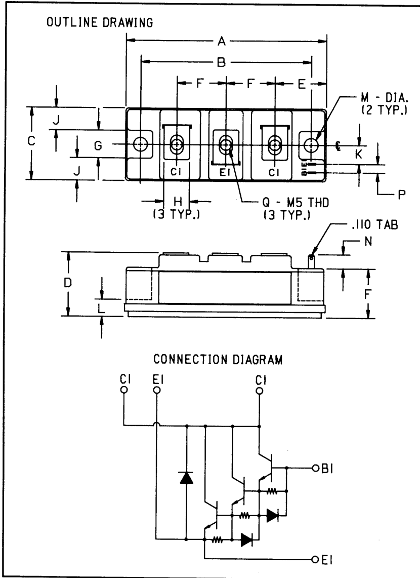
Outline Drawing
