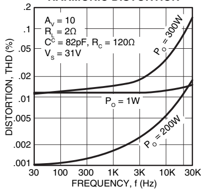
HARMONIC DISTORTION
