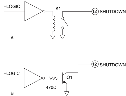
FIGURE 2. SHUTDOWN OPERATION
