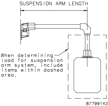
Load Diagram
