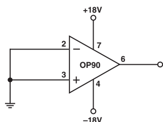
Figure 2. Burn-In Circuit
