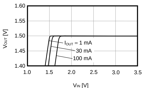
S-1701x15xx ( V_{OUT} = 1.5\text{ V} , T_a = 25^\circ\text{C} )
