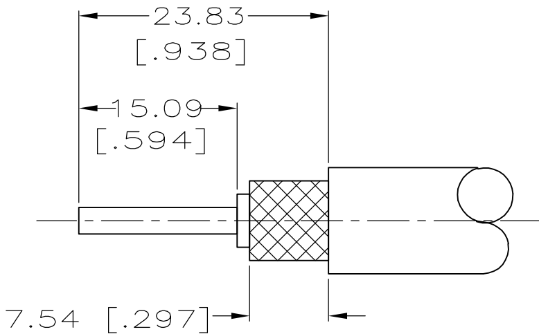
DETAIL A RECOMMENDED STRIP LENGTH
