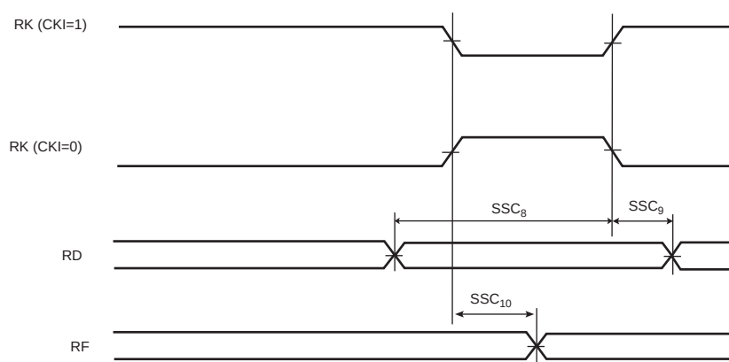
Figure 49-17. SSC Receiver, RK in Input and RF in Output
