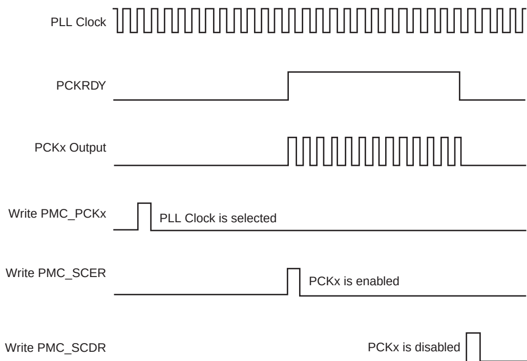
Figure 25-6. Programmable Clock Output Programming
