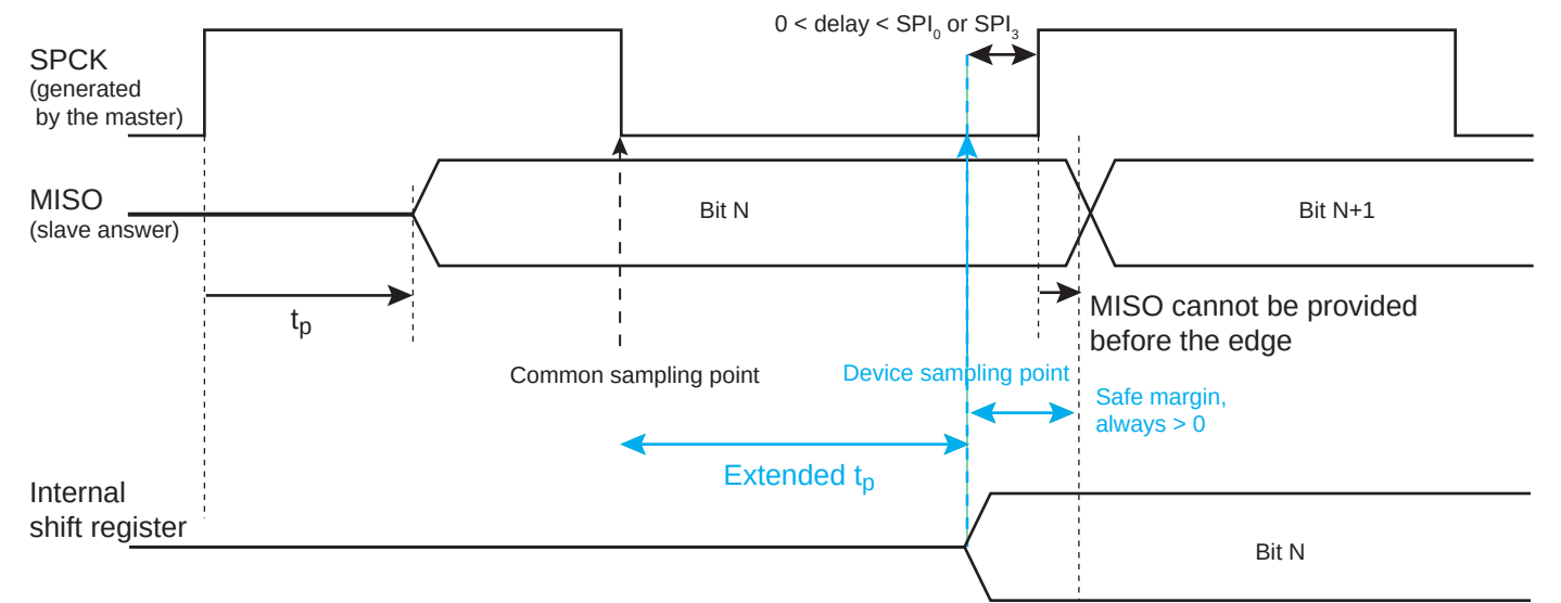
Figure 49-6. MISO Capture in Master Mode
