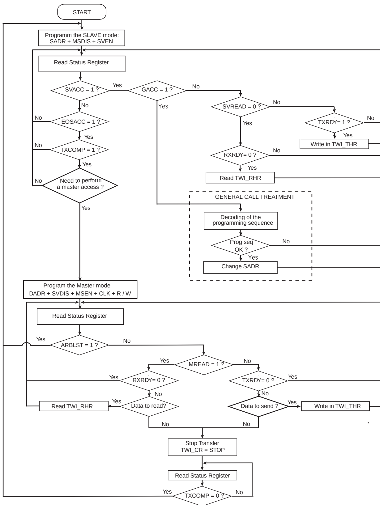
Figure 31-23. Multi-master Flowchart
