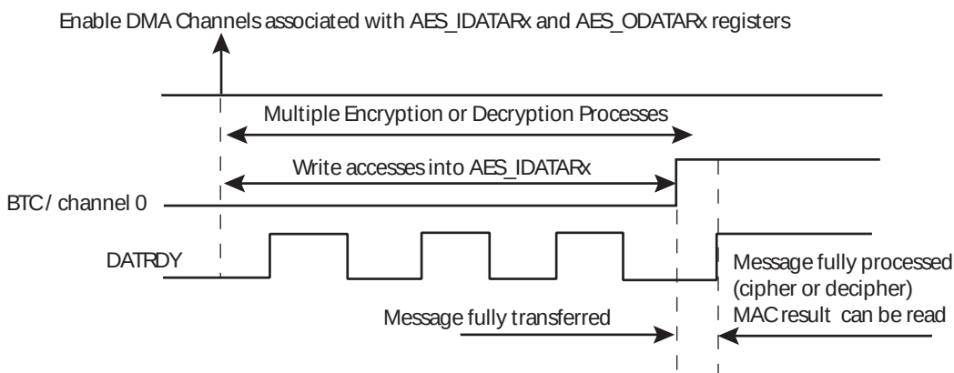
Figure 43-4. DMA transfer with LOD = 1
