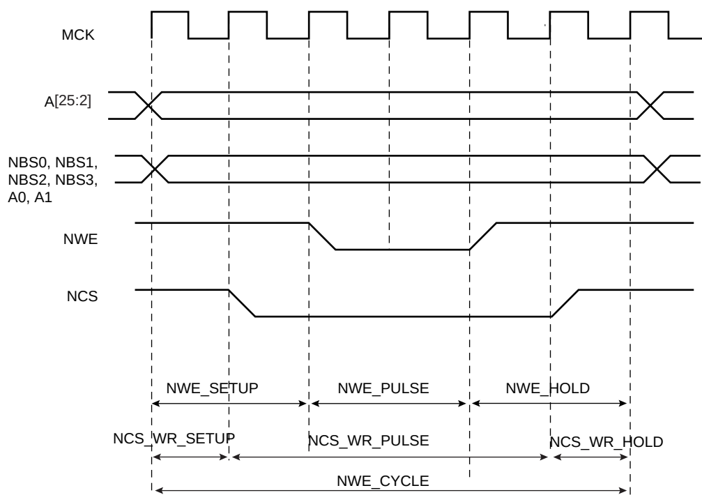
Figure 20-12. Write Cycle
