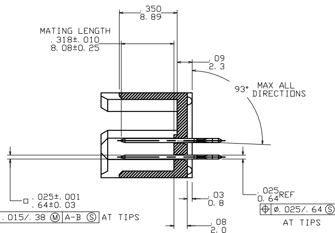
SECTION Y-Y
