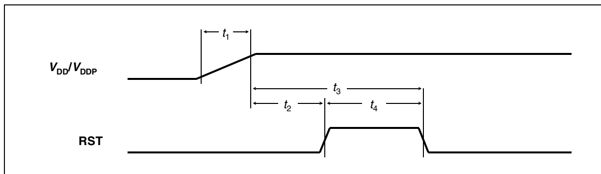
Figure 75 Reset Timing
