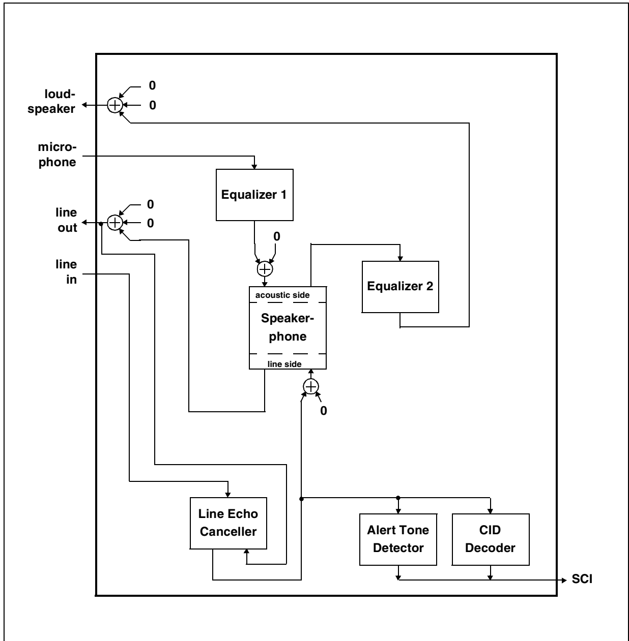
Figure 11 Functional Units - Speakerphone
