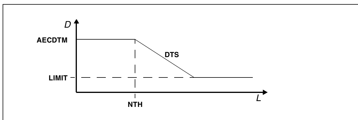
Figure 28 Double Talk Detection Adaptation
