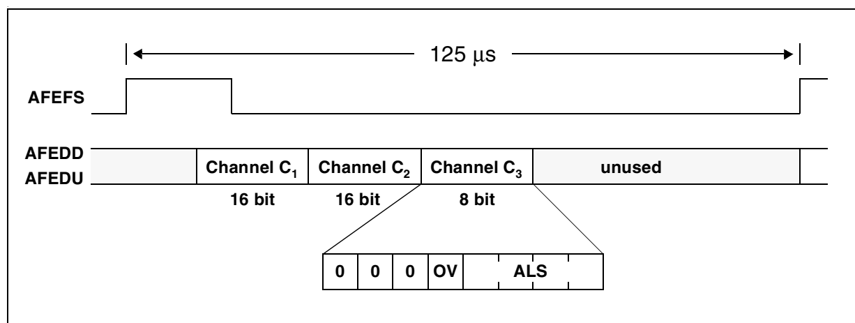
Figure 58 Analog Front End Interface - Frame Structure
