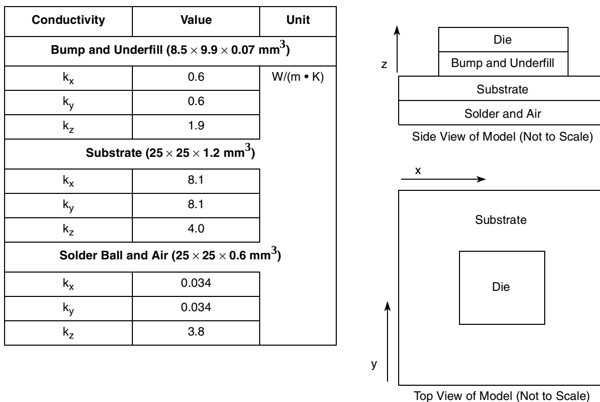
Figure 24. Recommended Thermal Model of MPC7447A
