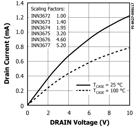
Figure 20. Output Characteristics.
