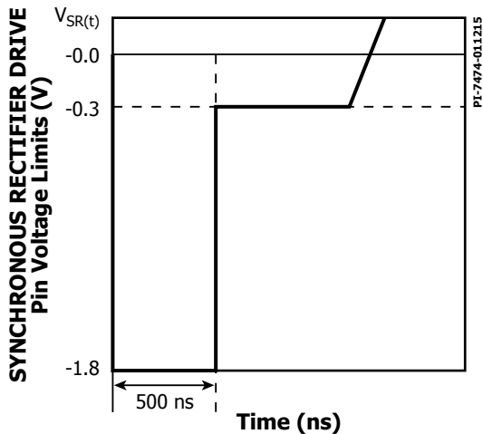
Figure 23. SYNCHRONOUS RECTIFIER DRIVE Pin Negative Voltage.
