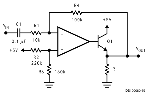
FIGURE 22. Power Amplifier
