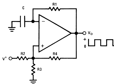
FIGURE 19. Squarewave Generator
