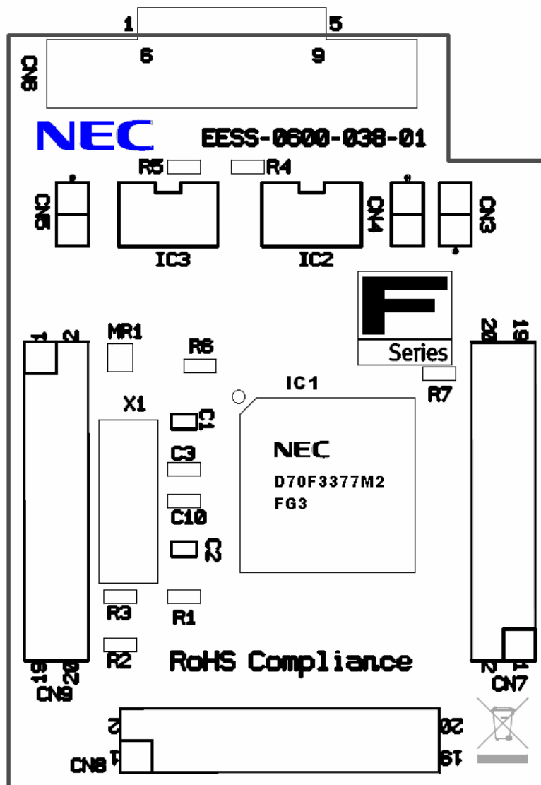
Figure 4: V850ES/Fx3 – CAN it! CPU module components
