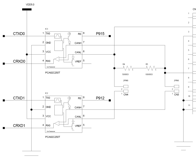
Figure 5: CAN transceivers
