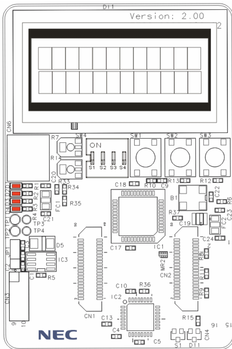
Figure 2: V850ES/Fx3 – CAN it! baseboard connectors, switches and LED's
