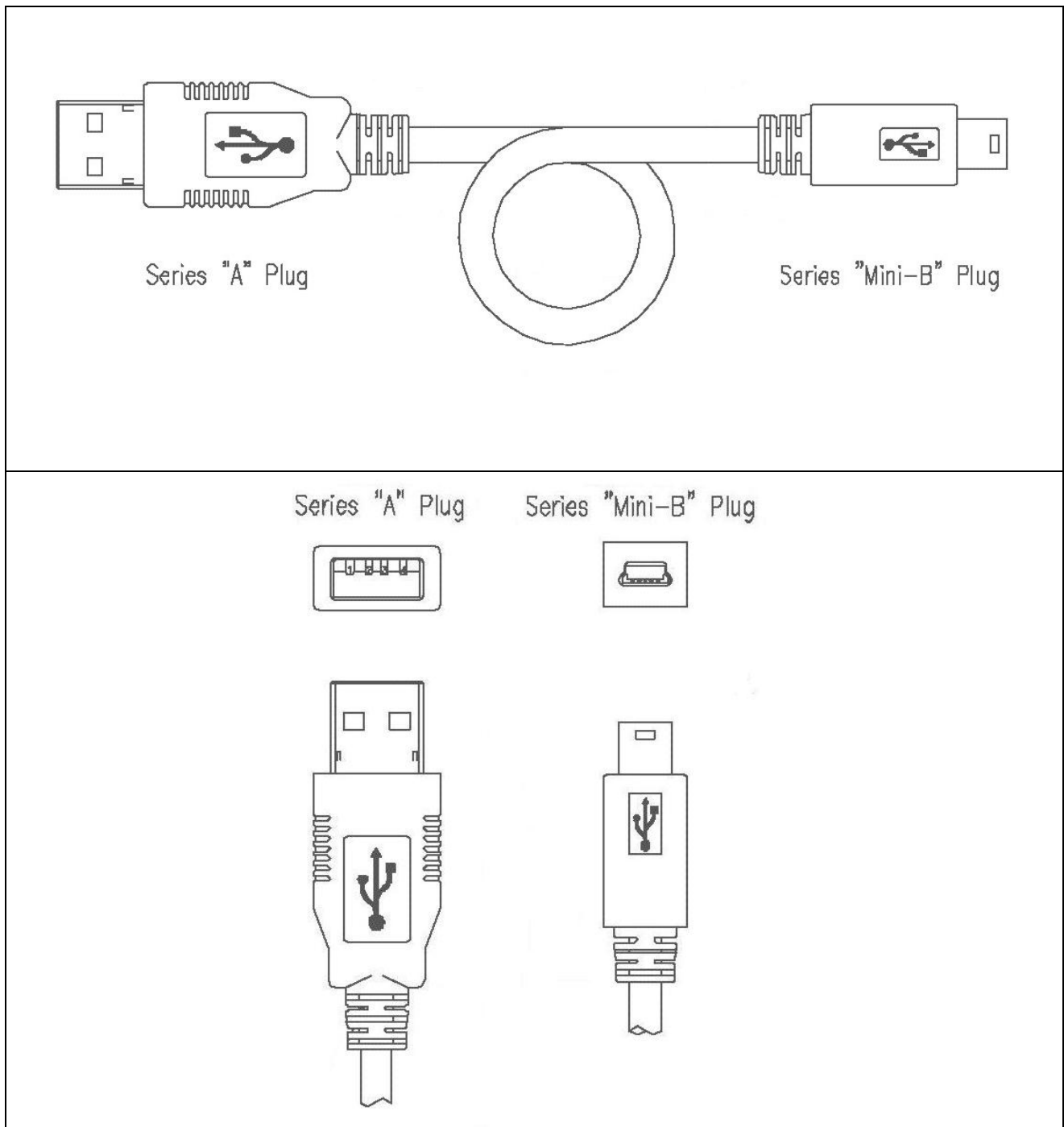
Figure 70: USB interface cable (Mini-B type)
