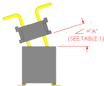
INITIAL X AXIS ANGULAR MISALIGNMENT
