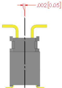
FINAL Y AXIS LINEAR MISALIGNMENT
