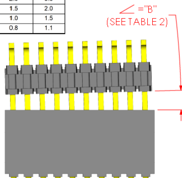
INITIAL Y AXIS ANGULAR MISALIGNMENT
