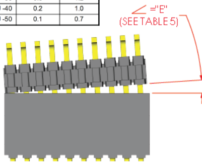
FINAL Y AXIS ANGULAR MISALIGNMENT
