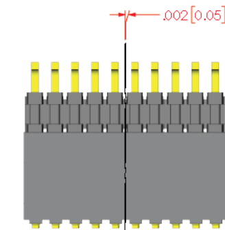
FINAL X AXIS LINEAR MISALIGNMENT
