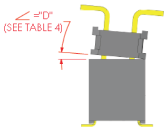
FINAL X AXIS ANGULAR MISALIGNMENT
