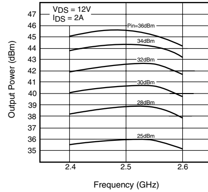
OUTPUT POWER vs. FREQUENCY
