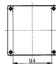
View F
