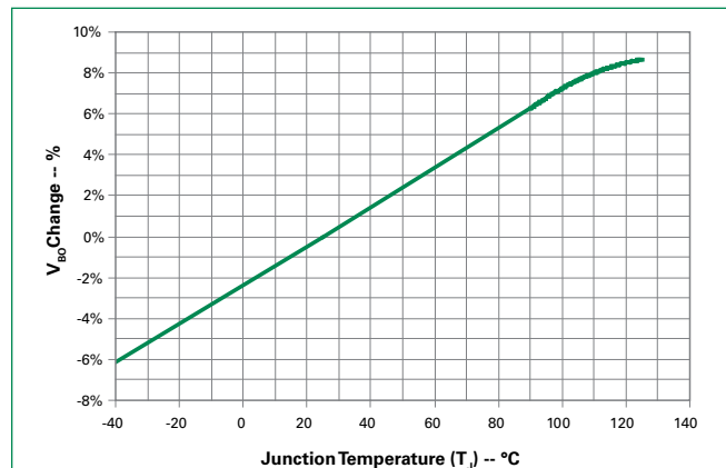
Figure 6: Normalized V_{BO} Change vs. Junction Temperature
