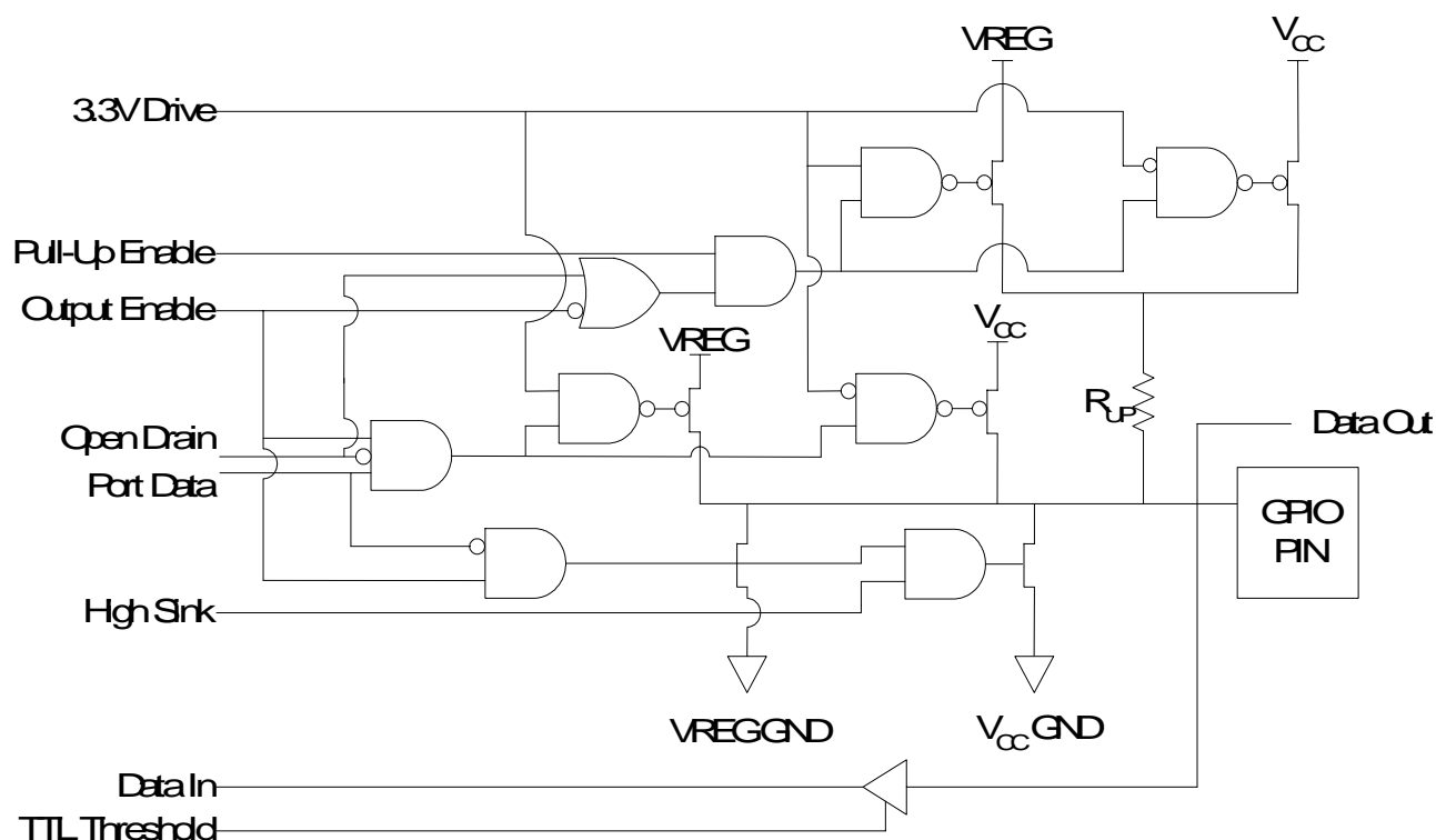
Figure 14-1. Block Diagram of a GPIO
