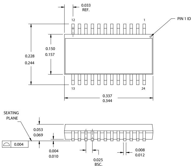
Figure 29-6. 24-lead QSOP O241
