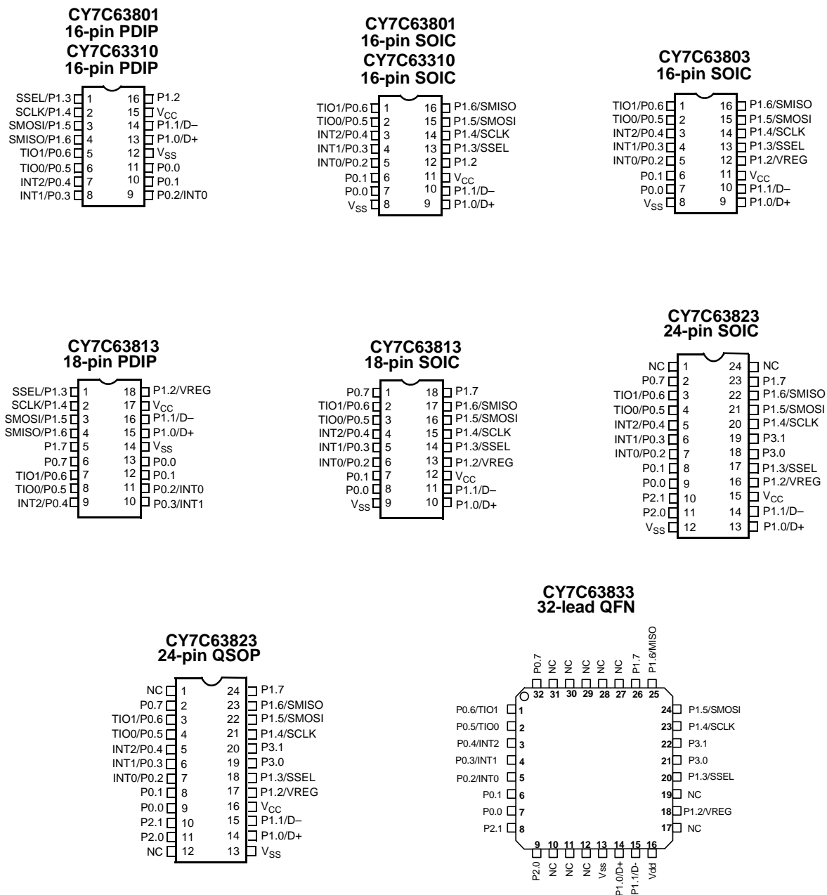
Figure 5-1. Package Configurations
