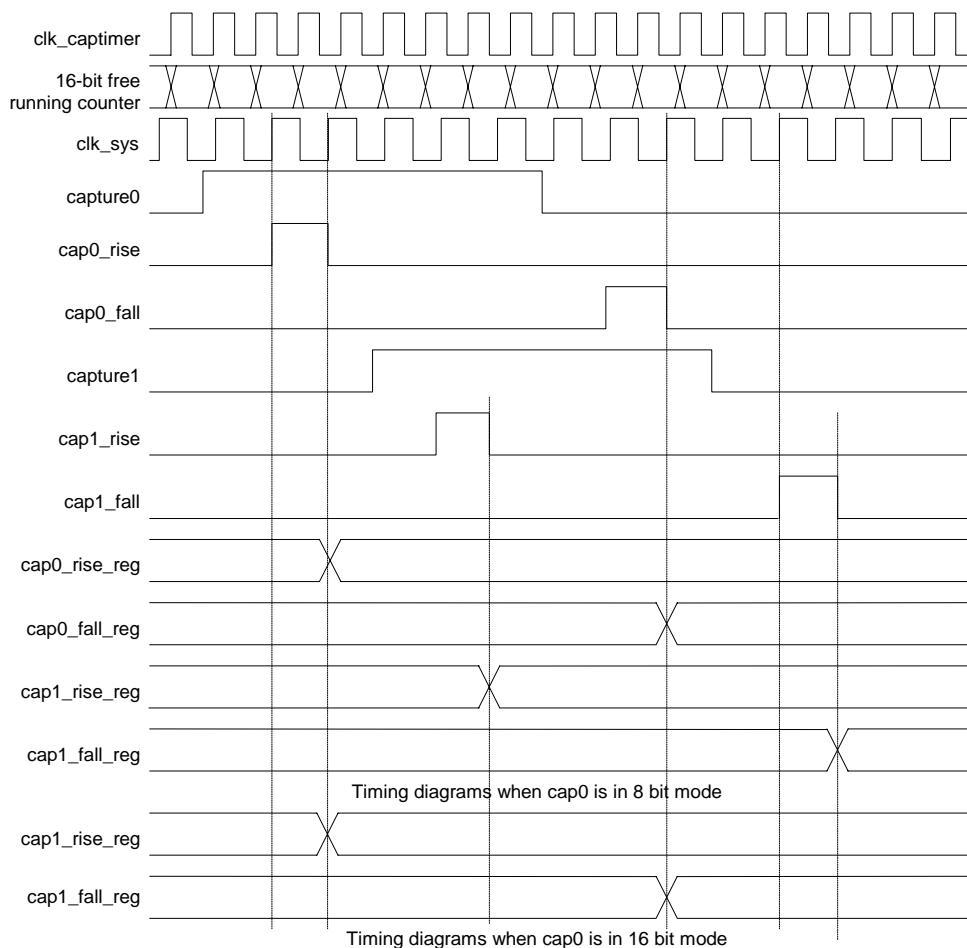
Figure 16-3. Timer Functional Timing Diagram
