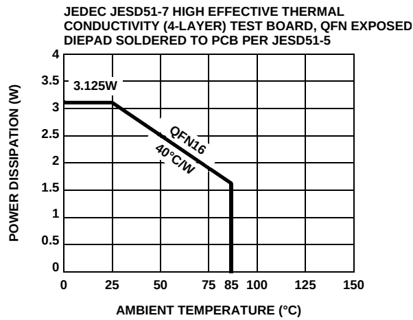
FIGURE 53. PACKAGE POWER DISSIPATION vs AMBIENT TEMPERATURE
