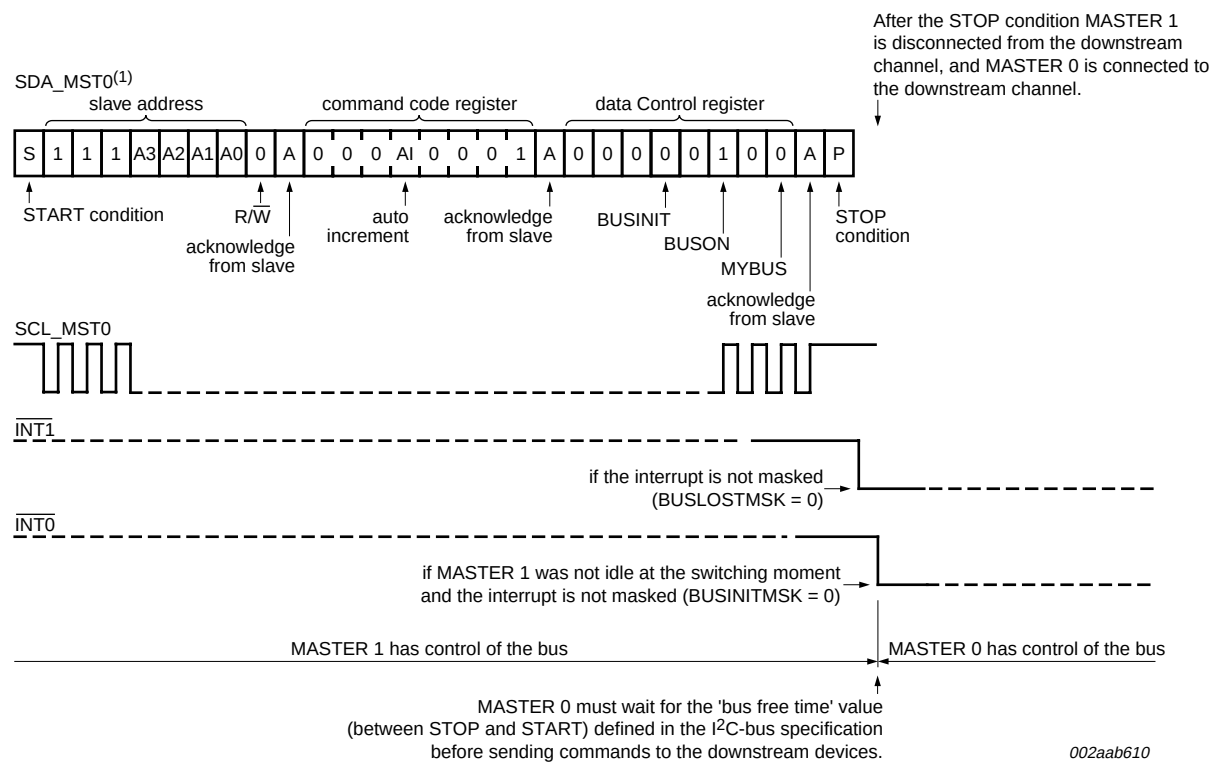
Fig 16. Write to the Control register and switch from Channel 1 to Channel 0 (bus recovery/initialization not requested)
