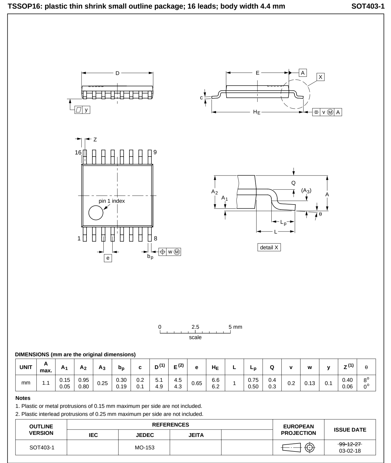
Fig 28. Package outline SOT403-1 (TSSOP16)
