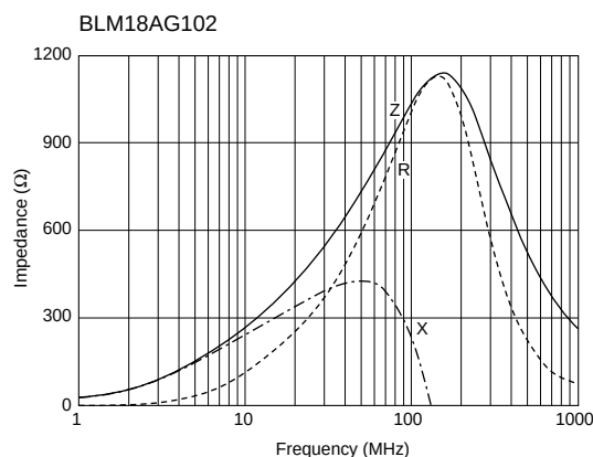
[Example of impedance frequency characteristics of inductor type EMIFIL®]
