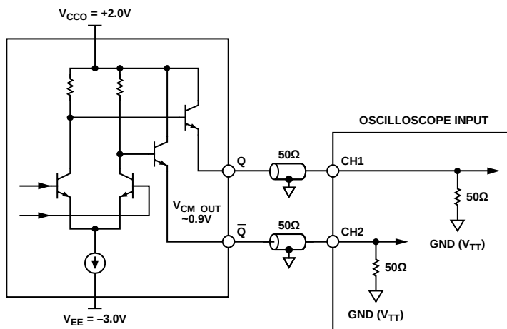
Figure 16. Output Interfacing Application Circuit, Output to Oscilloscope
