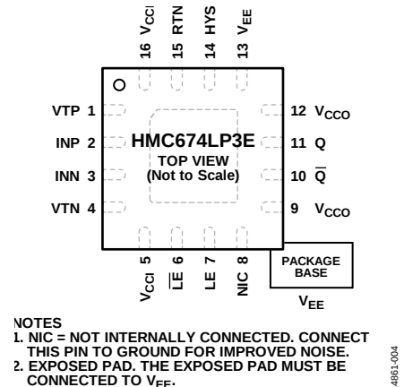
Figure 4. HMC674LP3E Pin Configuration
