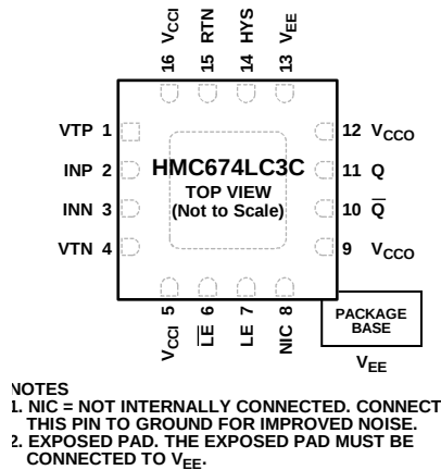
Figure 3. HMC674LC3C Pin Configuration
