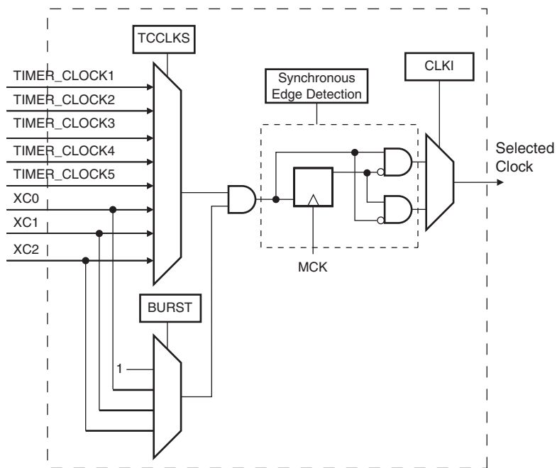
Figure 31-3. Clock Selection
