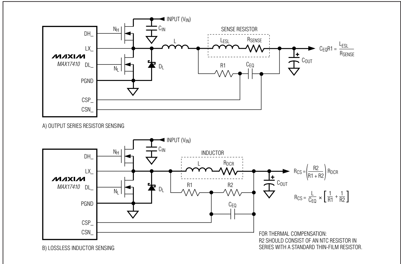
Figure 3. Current-Sense Methods
