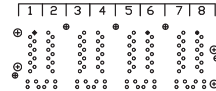
PORT ASSIGNMENT (COMPONENT SIDE VIEW)
