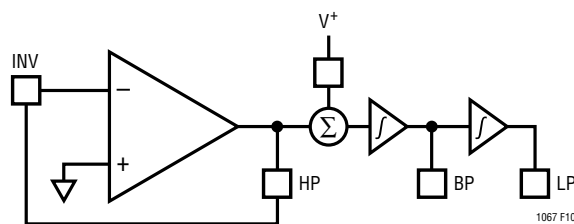
Figure 10. Connections for an Unused Section
