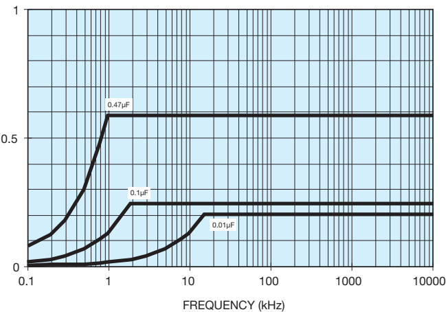
400 Vdc / 200 Vac
