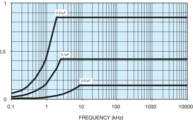
630 Vdc / 250 Vac
