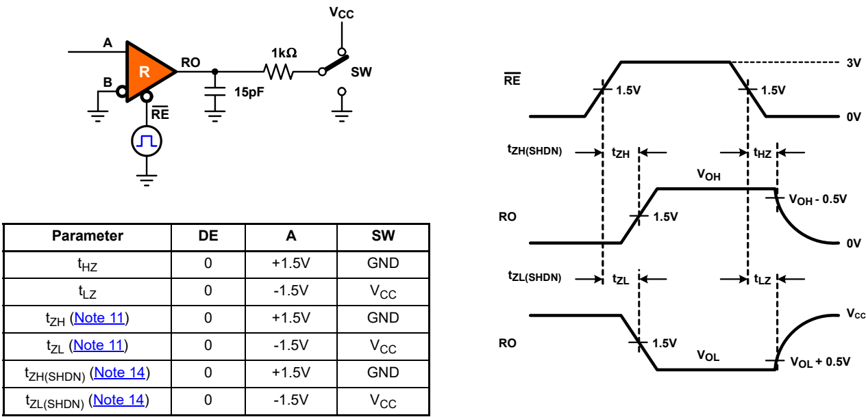
Figure 9. Measurement of Receiver Enable and Disable Times
