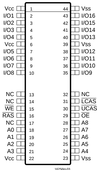
40/44 Pin Plastic TSOP-II PIN CONFIGURATION Top View
