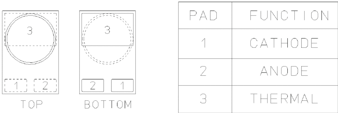
Figure 2. Pad configuration.
