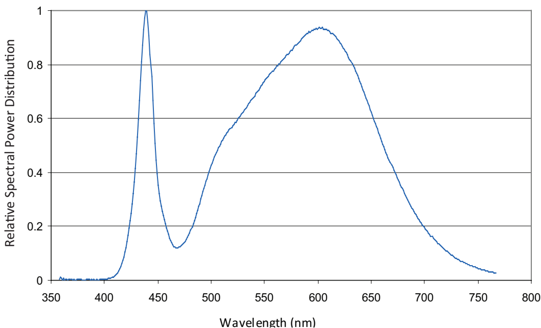
Figure 7. Color spectrum of 3500K emitters, integrated measurement.
