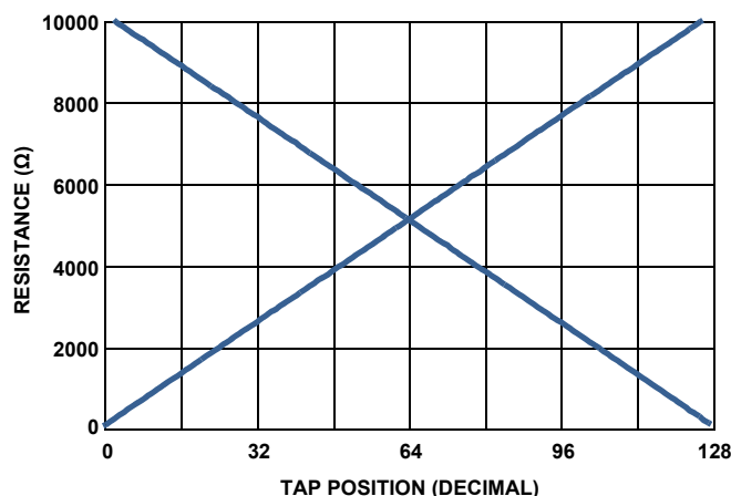
FIGURE 1. FORWARD AND BACKWARD RESISTANCE vs TAP POSITION, 10k DCP
