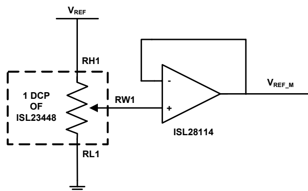
FIGURE 2. V_{\text{REF}} ADJUSTMENT
