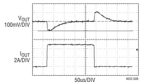
12V to 2.5V Load Step Response
