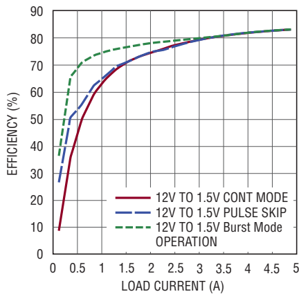
Light Load Efficiency
