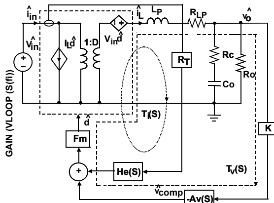
FIGURE 49. SMALL SIGNAL MODEL OF SYNCHRONOUS BUCK REGULATOR
