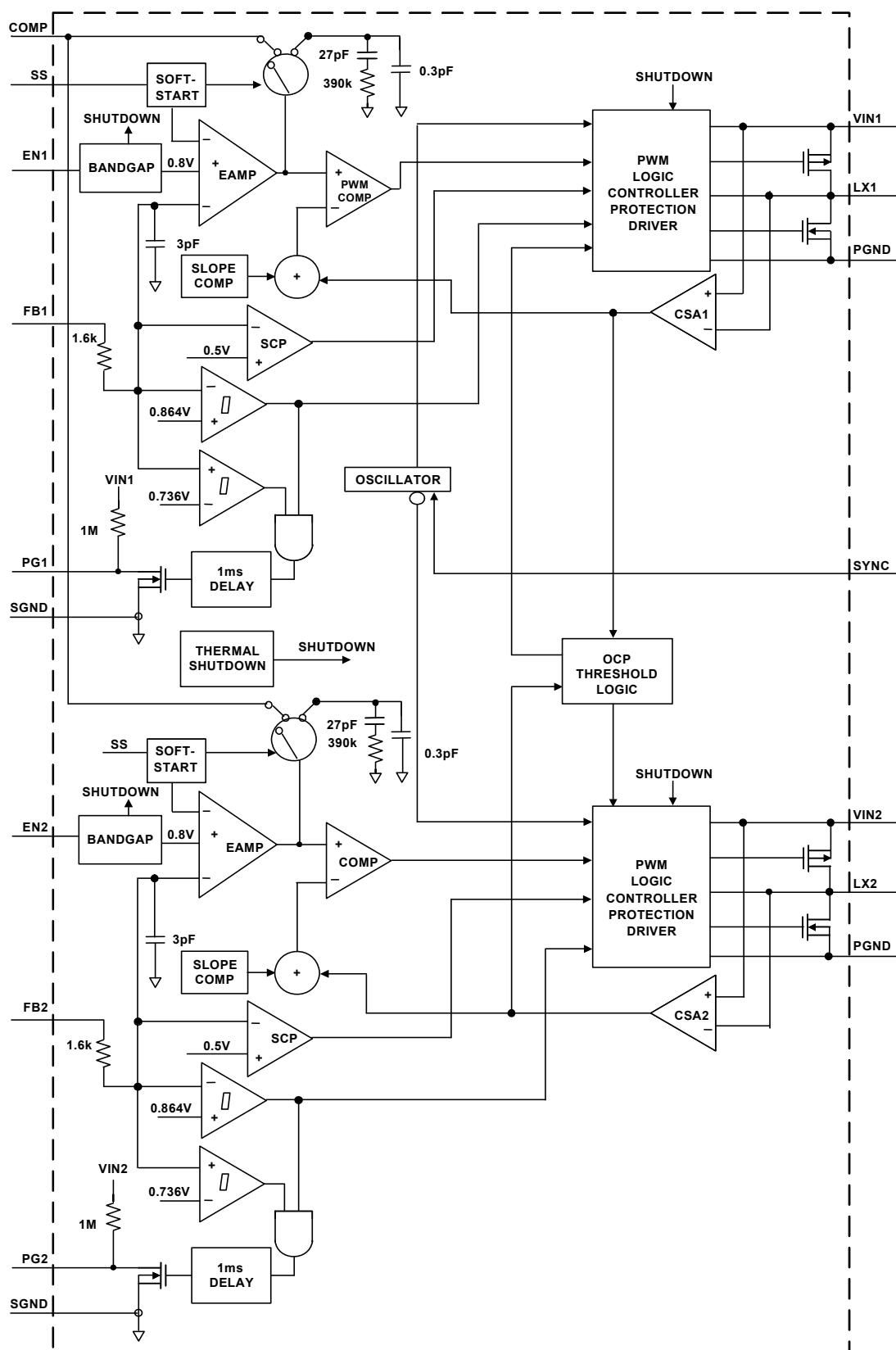
FIGURE 5. BLOCK DIAGRAM
