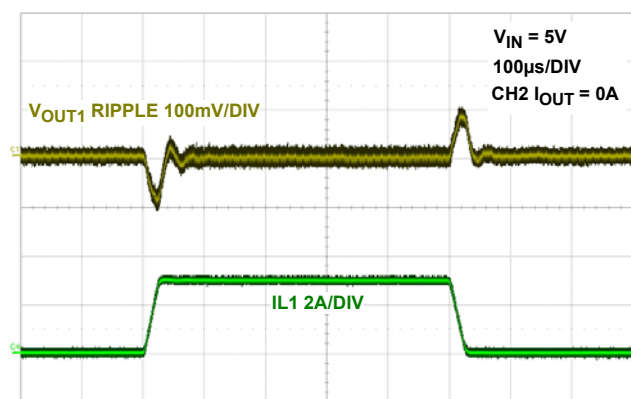
FIGURE 15. LOAD TRANSIENT CHANNEL 1
