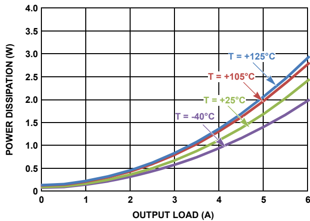
FIGURE 37. POWER DISSIPATION, V_{IN} = 3.3\text{V} , V_{OUT} = 1.8\text{V}
