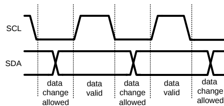
Figure 24. I 2 C Signals: Data Validity
