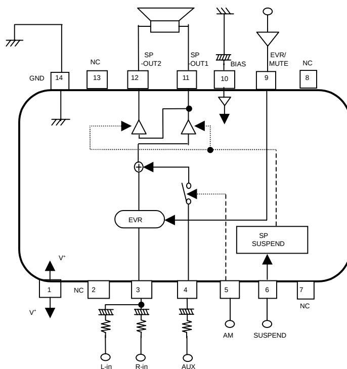
NJM2166 E/V Block Diagram
