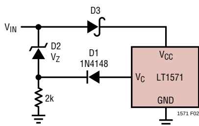
Figure 2. Undervoltage Lockout
