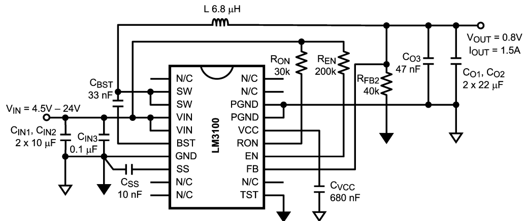
Typical Application Schematic for V_{OUT} = 0.8V
