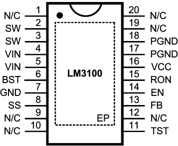
20-lead Plastic eTSSOP (MXA20A)
