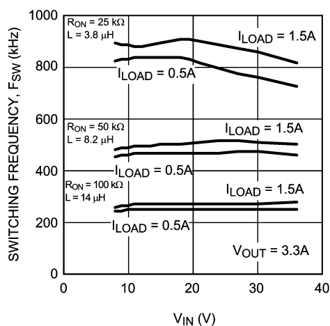
Switching Frequency, F_{SW} vs V_{IN}
